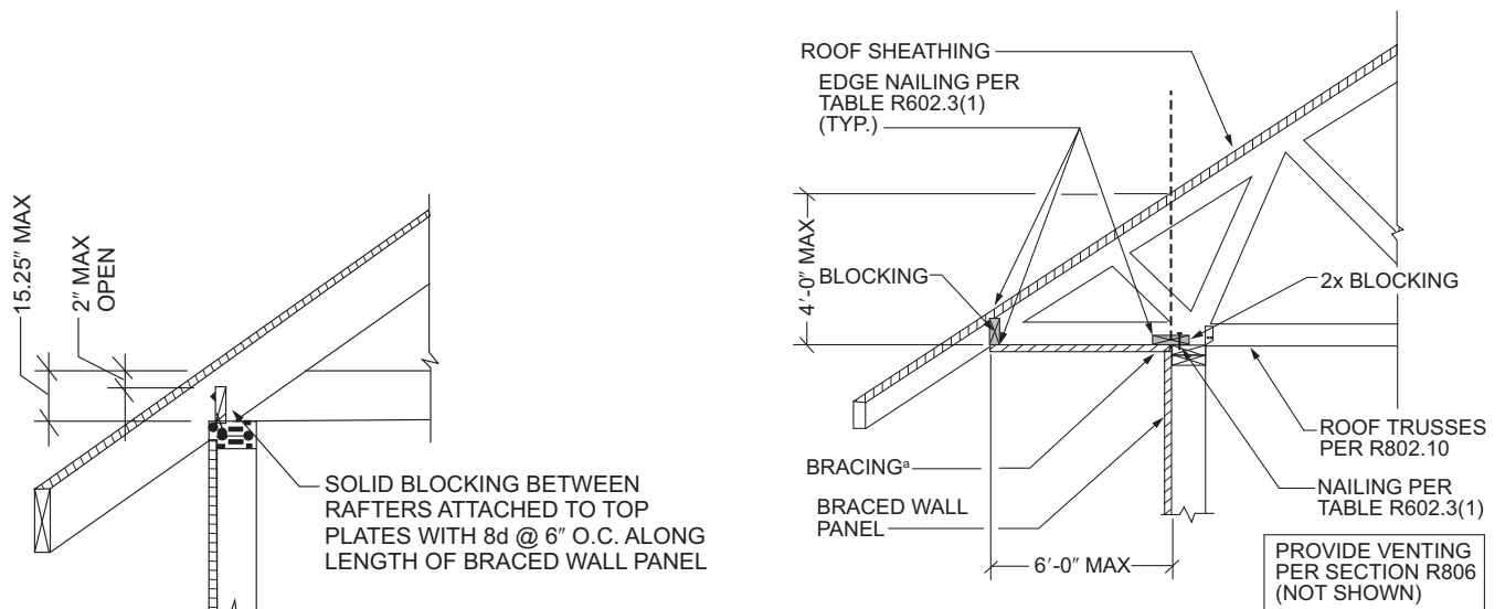
FIGURE R602.10.8(2) BRACED WALL PANEL CONNECTION WHEN PARALLEL TO FLOOR/CEILING FRAMING
