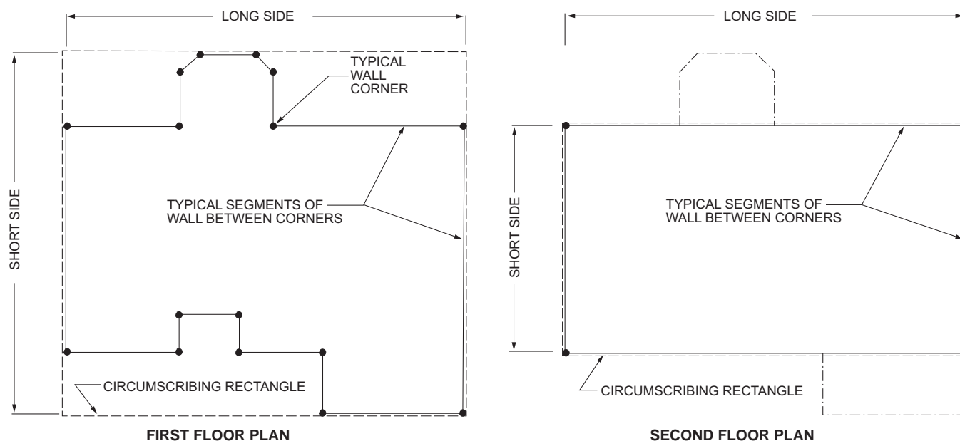
FIGURE R602.12.1 RECTANGLE CIRCUMSCRIBING AN ENCLOSED BUILDING
