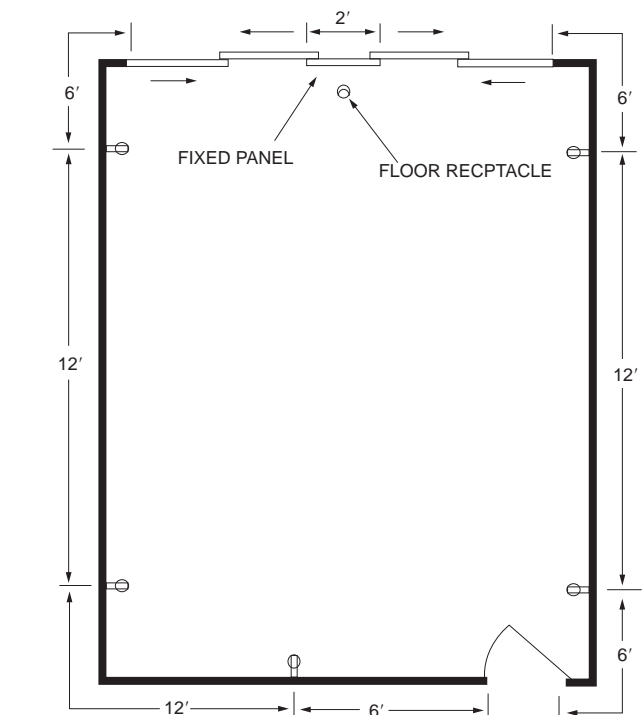
FIGURE E3901.2 GENERAL USE RECEPTACLE DISTRIBUTION
